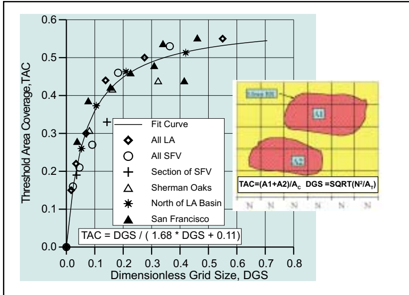
■ Figure 1. Hyperbolic Fit for Threshold Area Coverage and Dimensionless Grid Size for Pipeline Damage Patterns (Toprak, et al., 1999)
